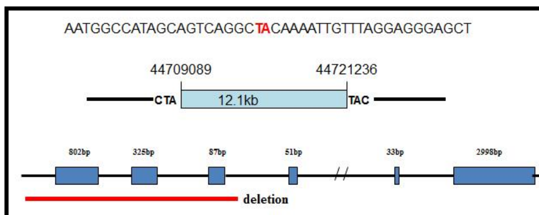
Figure 5: Sequencing result of selected samples. All three sequencing results showed the same sequence at the deletion breakpoint (red colour letters) at 44,709,089bp and 44,721,236bp (middle). The bottom figure shows a schematic illustration indicating that the deletion removes exon 1-3 of HMGA2 gene; dark blue rectangles mean exons.
