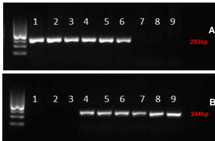
Figure 7: Genotyping results. Sample 1-3: PNT9, PNT10, PNT 11(peanut); Sample 4-6: NDA39, NDA41, NDA50 (dwarf); Sample 7-9: PST7, PST10, PST16 (wild type). A) PCR amplicons of Peanuts and dwarfs with P1+P2 were 293bp; no amplicons of wild type rabbits; B) PCR amplicons of dwarfs and wild type rabbits with P1+P3 were 244bp; no amplicons of Peanuts.
