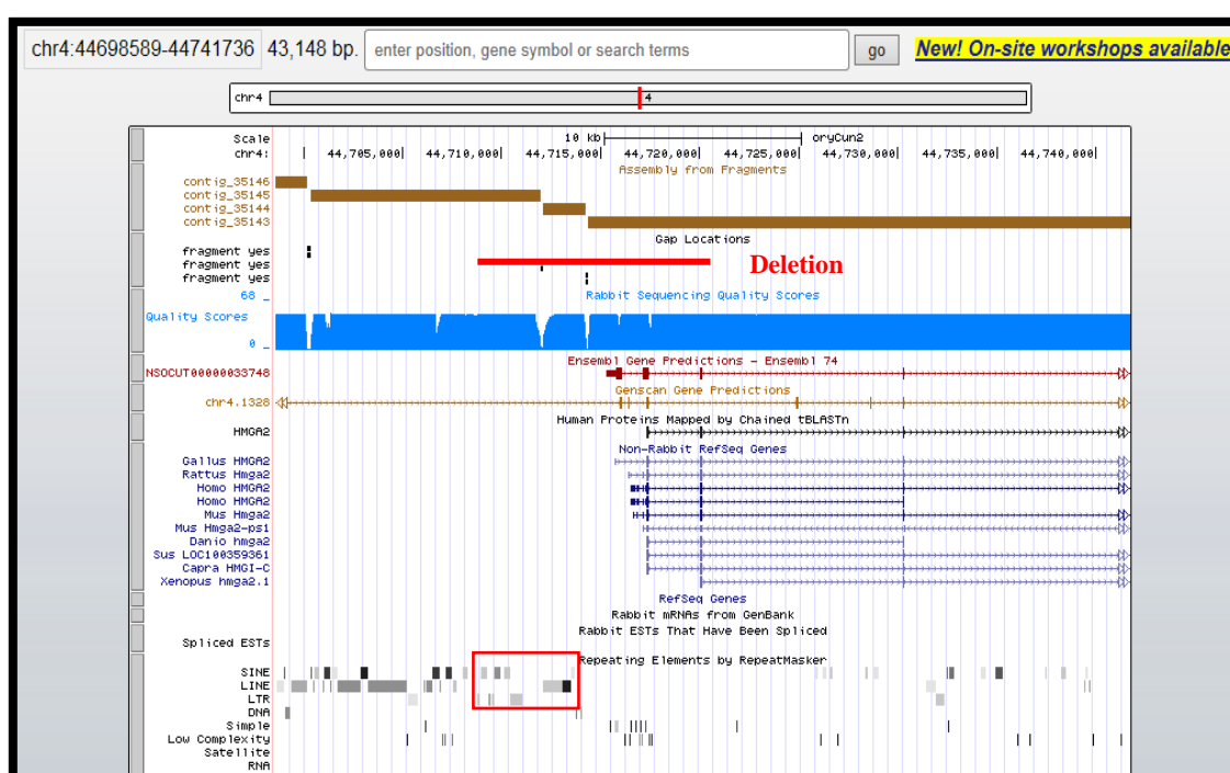
Figure 6: Genomic structure at the deletion site illustrated using the UCSC genome browser.
