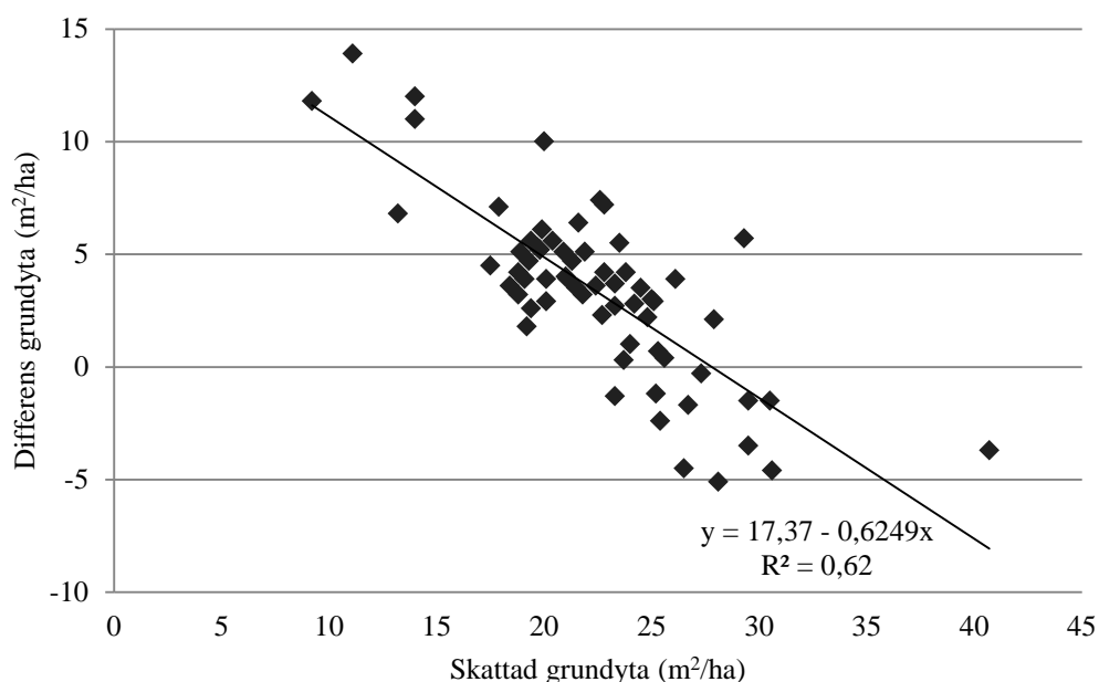
Figur 6. Differens i grunddyta ( \text{m}^2/\text{ha} ) som en funktion av skattad grunddyta vid objektiv inventering. Figure 6. Differences in basal area ( \text{m}^2/\text{ha} ) as a function of estimated basal area in the objective survey.
