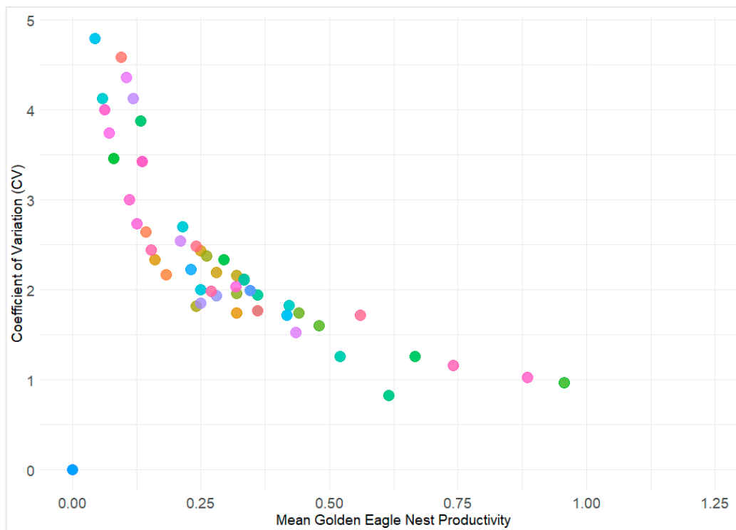
Figure 7. Relationship between mean nest productivity and its variation for golden eagles in Västerbotten.
