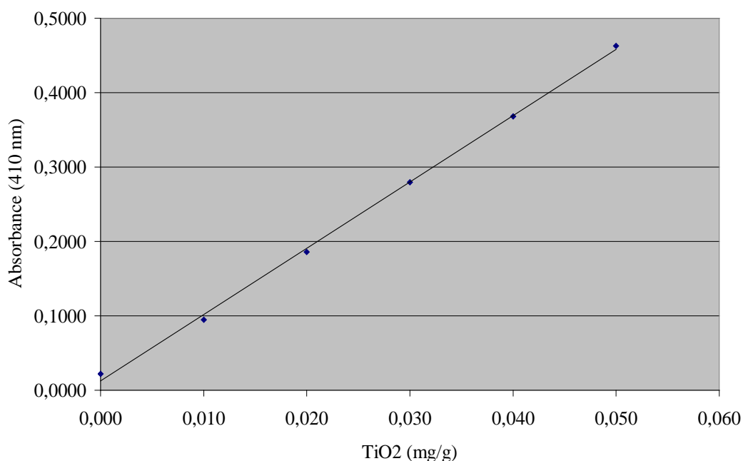
Figure 5. The standard curve applied in TiO 2 determinations ( r^2=0.9987 ).
